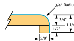
* KITCHEN AND VANITY TOP WFB-22 1/2 S WFK-25 S
