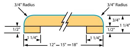
BAR TOP WFB-12 WFB-15 WFB-18
