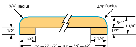
BAR TOP WFB-26 WFB-27 1/2 WFB-30 WFB-36 WFB-42
