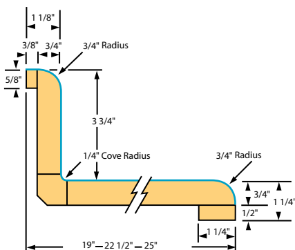
KITCHEN AND VANITY TOP WFB-19 WFB-22 1/2 WFK-25
